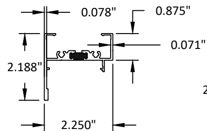
7 FIXED SNAP COVER 6063-T5
