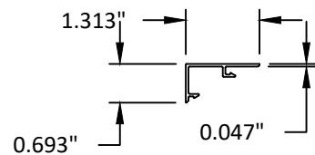
7 FIXED SNAP COVER 6063-T5
