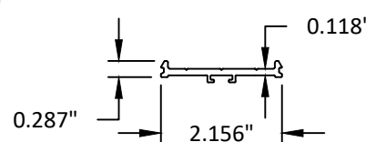
5 PRESSURE BAR 6063-T5
