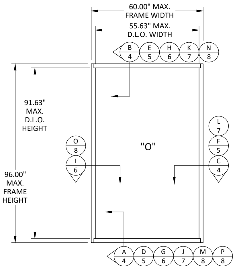
ELEVATION - B SINGLE TESTED UNIT
