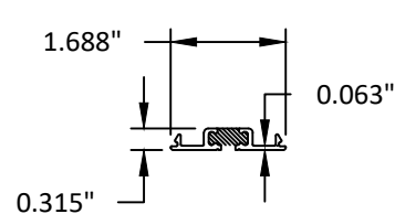
26 THROUGH FRAME FILLER PLATE 6063-T5
