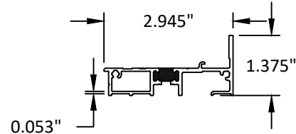
3 2-1/4\" WEeping SILL FLASHING 6063-T5
