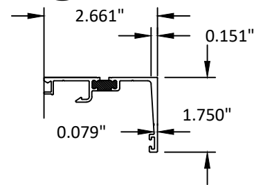
4 RECEPTOR 6063-T5
