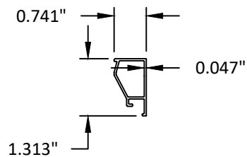
32 1 1/4\" X 1\" COVER 6063-T5
