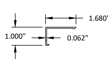
53 4\" SILL TRIM 6063-T5
