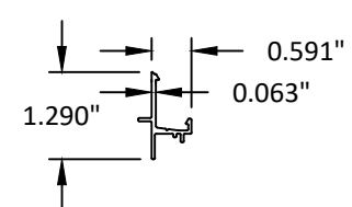
6 FIXED GLASS STOP 6063-T5
