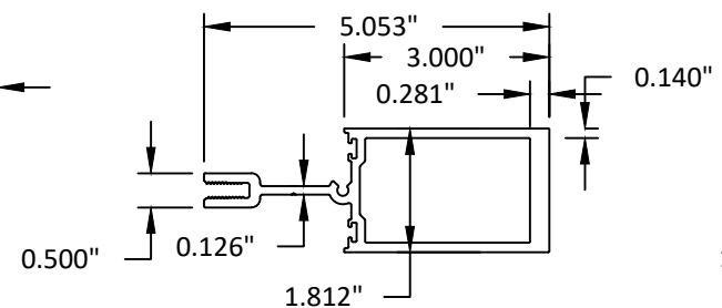
10 STACKING MULLION 6063-T5
