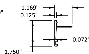
11 RECEPTOR STOP 6063-T5
