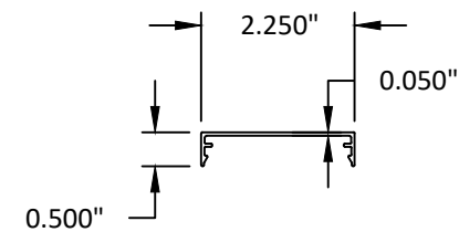
12 COVER 6063-T5
