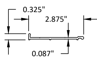
9 SILL TRIM BASE 6063-T5
