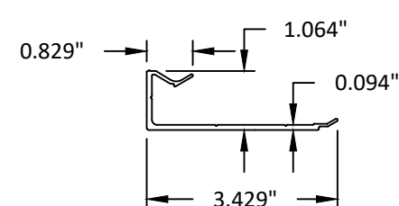
53 4\" SILL TRIM 6063-T5
