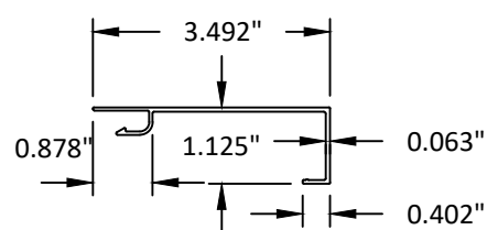
37 1 1/8\" X 3 1/2\" COVER 6063-T5
