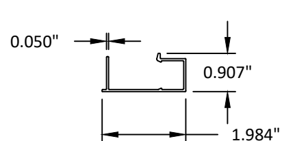
38 STRAP ANCHOR 6063-T5 MINIMUM 4 1/2\" LENGTH
