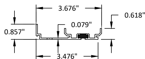
38 STRAP ANCHOR 6063-T5 MINIMUM 4 1/2\" LENGTH
